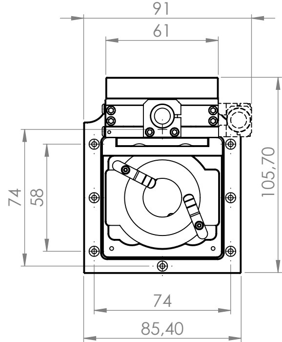
(Optional) Side-Mounted Actuator
